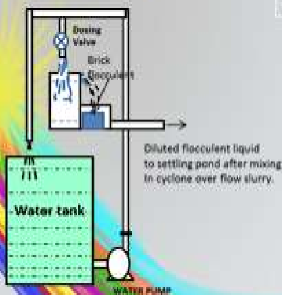
FLOCCULENT DISOLUTION & DOSING SYSTEM
